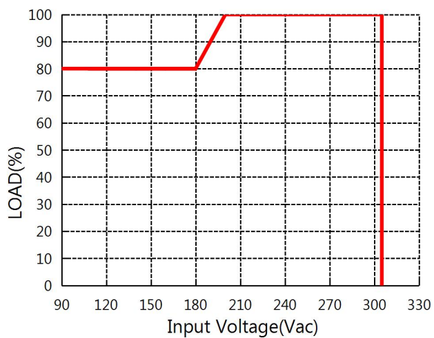
Fig.7 Output Power VS Input Voltage
